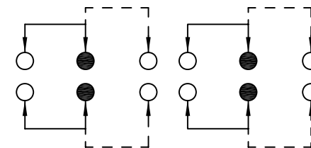
SCHEMATIC (NON-SHORTING)
